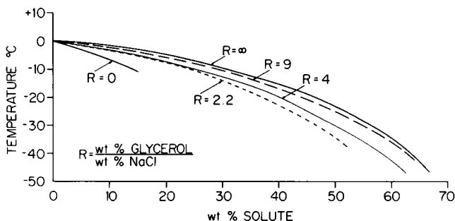
FIGURE 2 Equilibrium phase-diagram for the ternary system NaCl-glycerol- H_2O . The graph shows the freezing point as a function of the total solute concentration (weight percent) for solutions with the indicated R value (glycerol:NaCl weight ratio), plotted from the data of Goldston (1974) and Shepard et al. (1976).
